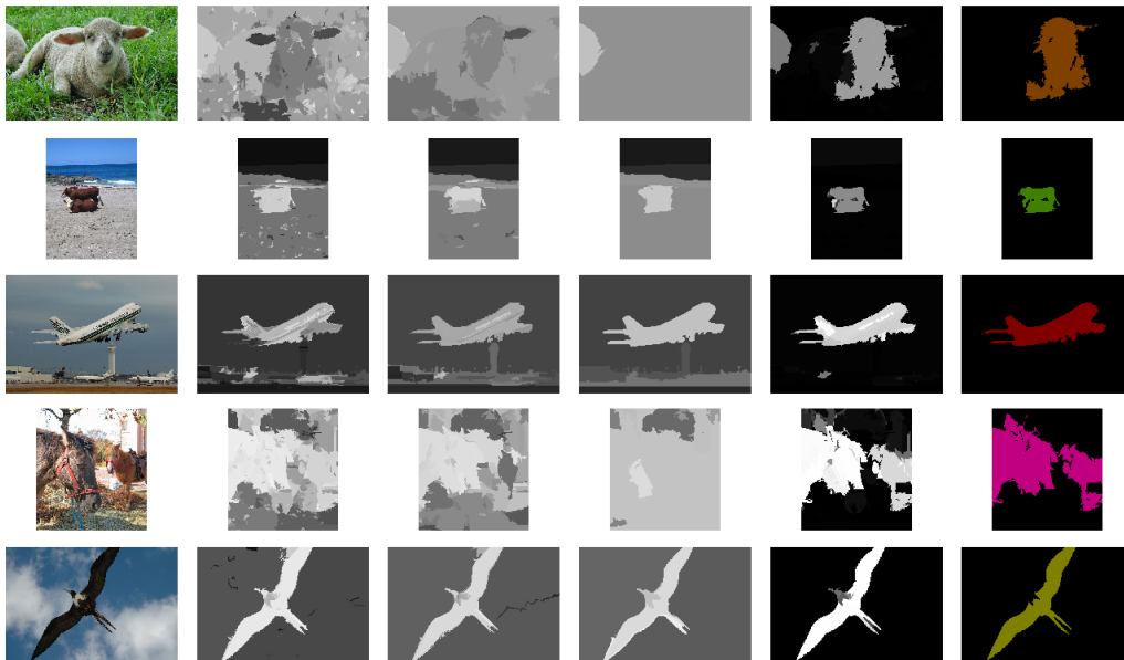
Figure 4. Demonstration of spatial smoothing with Conditional Random Fields (CRF) and segmentation (a) Sample input images. (b)-(d) Confidences of local classifiers for patches p for the layers l = 1 \dots 3 , i.e. from fine to coarse layers. Only the output of the classifier for which the posteriors after belief propagation are the highest are shown. (e) Posteriors on leaf layer (finest) after belief propagation (f) Applying a global threshold on the posteriors and assigning each segment with the maximum marginal probability yields the final semantic segmentation.
